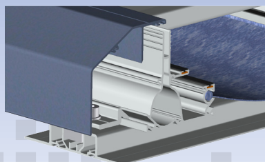
Side rafter
