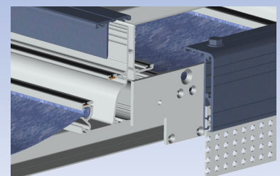
Central rafter
