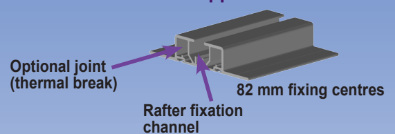
Support rail
